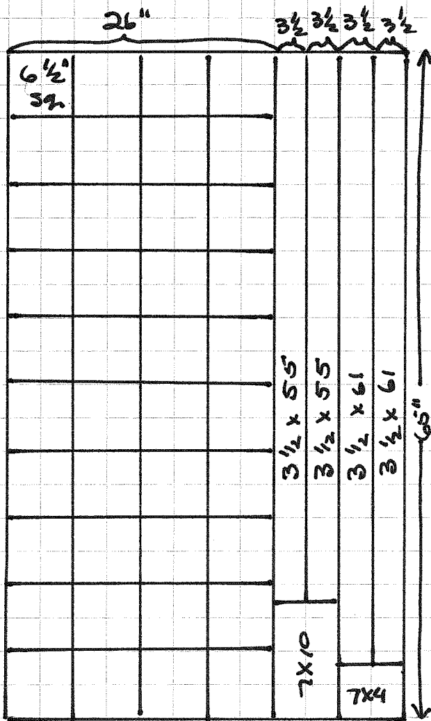
Block & Border Cutting Layout
